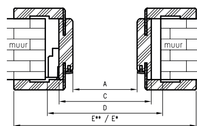
Horizontale doorsnede OR/ORC
