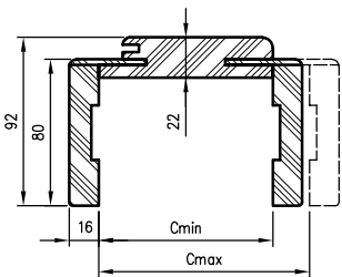
Horizontale doorsnede OF
