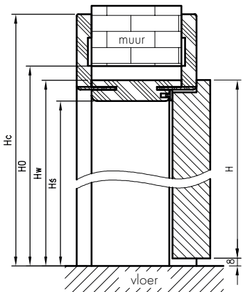
Verticale doorsnede OF
