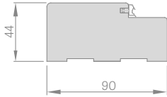
Vast frame
